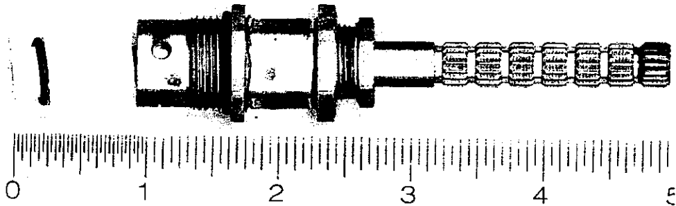
Auburn Brass tub & shower compression (washerless) stem with nylatron seat*2-40092-001*HOT*2-40092-002*COLD
