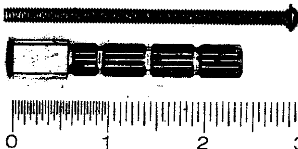
Auburn Brass extension (slip-over)**2-210-002 NOTE:Make sure althread will slip over this extension small 16 point broach
