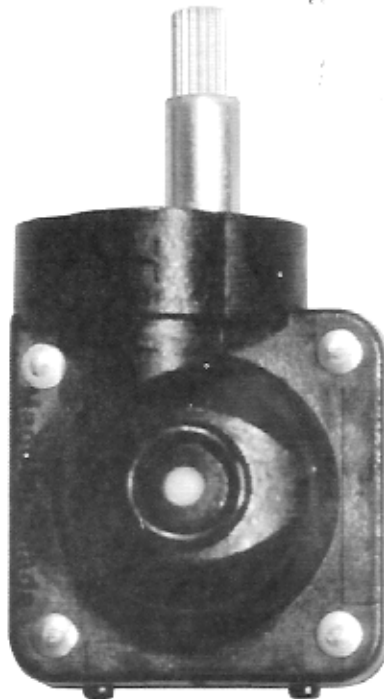
062N1285 Pressure Balancing Cartridge
